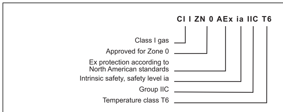
Fig. 9 Example: US identification according to NEC 505
