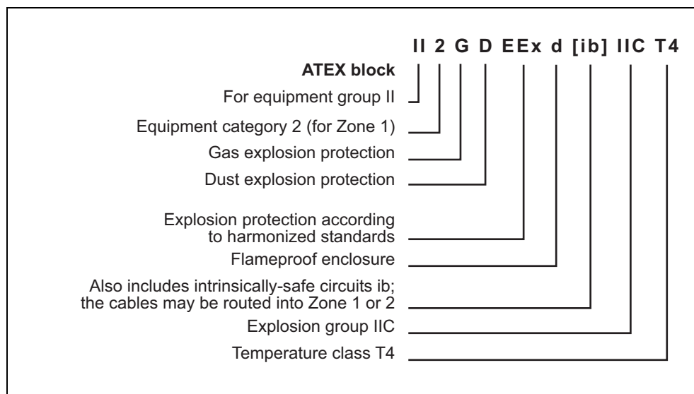
Fig. 6 Example: explosion-proof equipment
