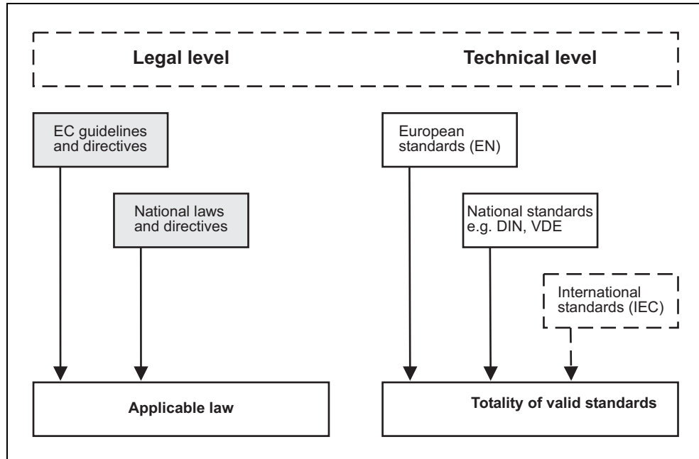
Fig. 1 Legal considerations of explosion protection in Europe
