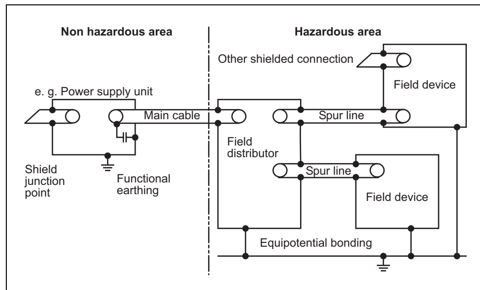
Fig. 15 PROFIBUS PA earthing
