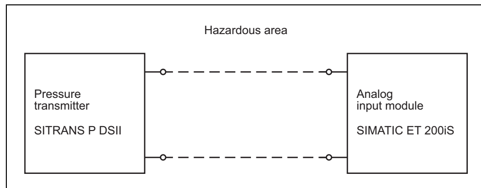
Fig. 12 Connection of a pressure transmitter to an analog input module
