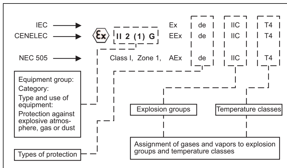
Fig. 4 Identification according to IEC / CENELEC / NEC 505
