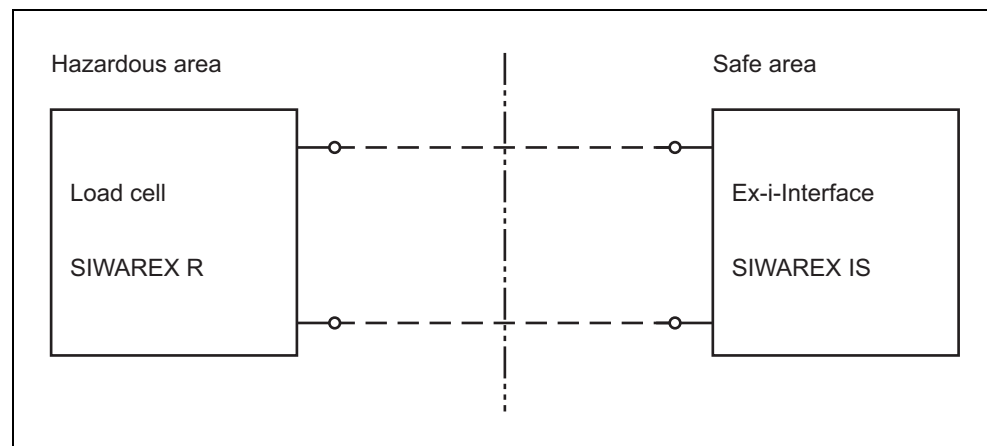
Fig. 13 Connection of a SIWAREX R load cell with a SIWAREX IS Ex-i interface
