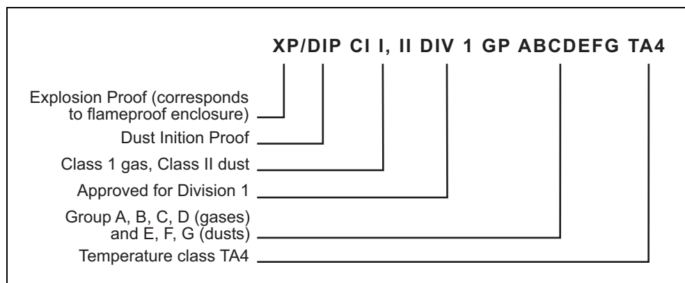
Fig. 8 Example: US identification according to NEC 500
