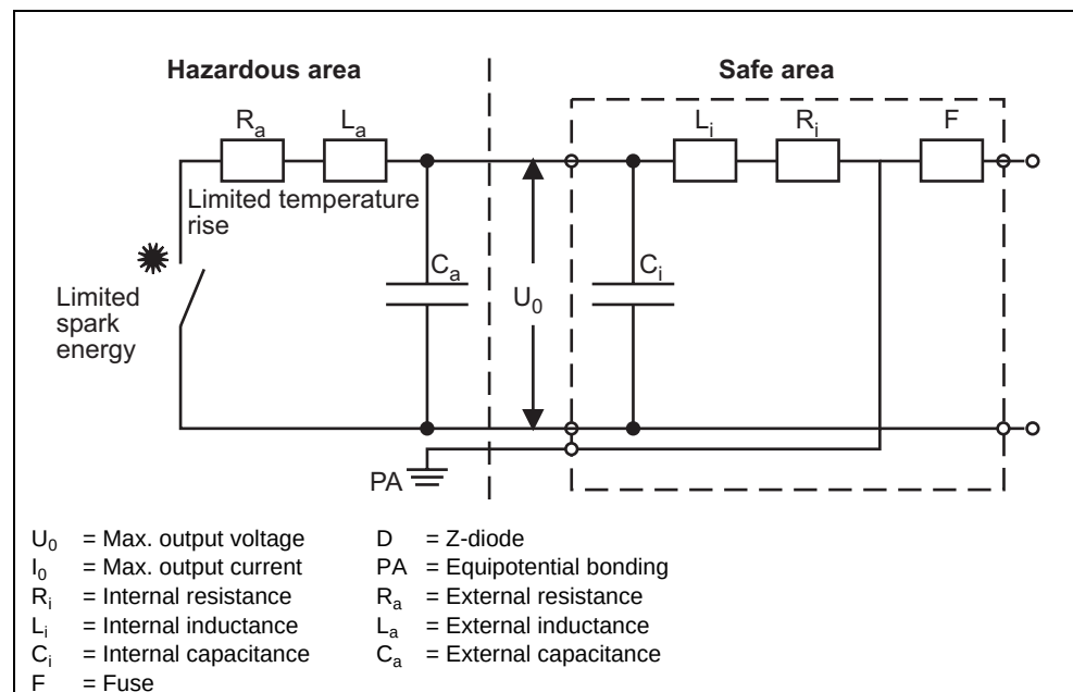
Fig. 10 Block diagram for voltage/current limiting with type of protection "Intrinsic safety"
