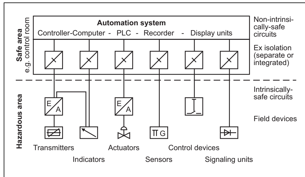
Fig. 11 Typical design of an intrinsically-safe measurement and control system
