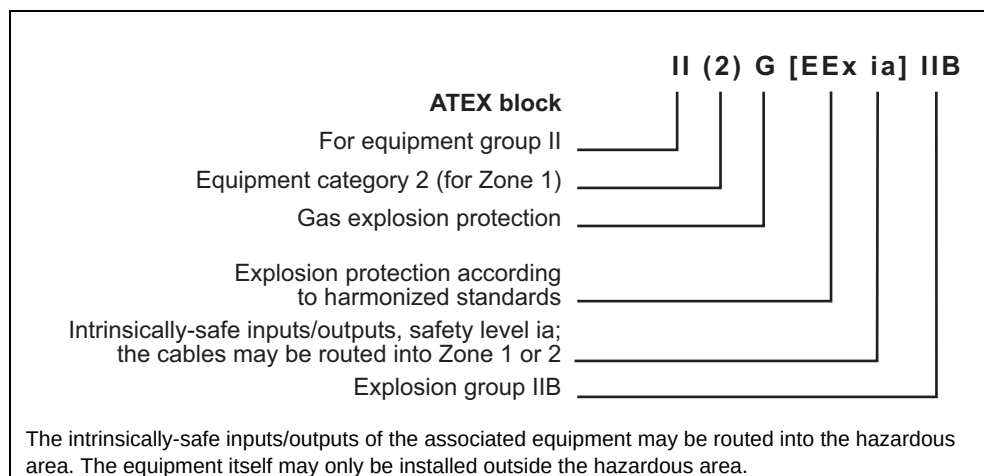
Fig. 7 Example: associated equipment
